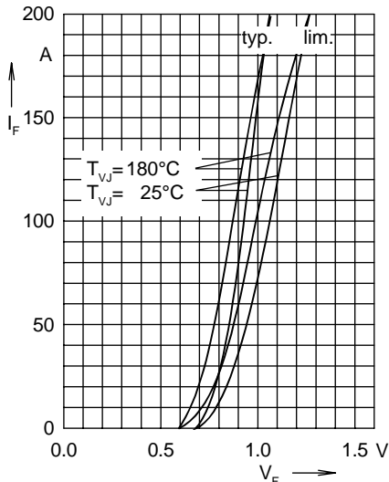
Fig. 1 Forward characteristics
